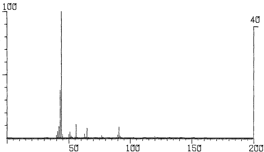
FIG. 3—The typical electron impact mass spectrum of amphetamine.
