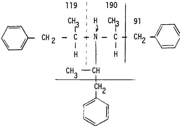
FIG. 7—The fragmentation scheme of tri-(1-isopropylphenyl)-amine.
