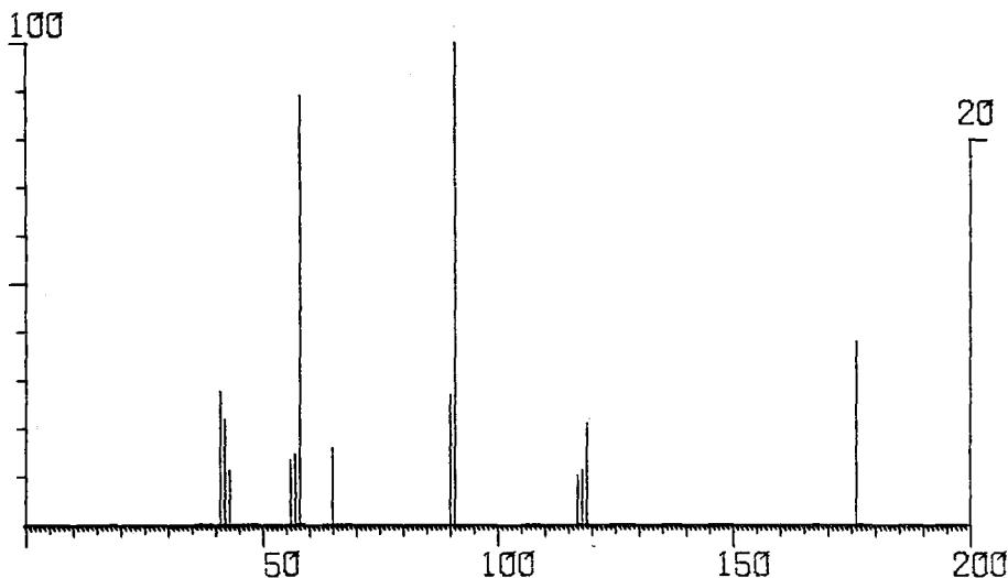
FIG. 12—The mass spectrum of di-(1-isopropylphenyl)-methylamine.
