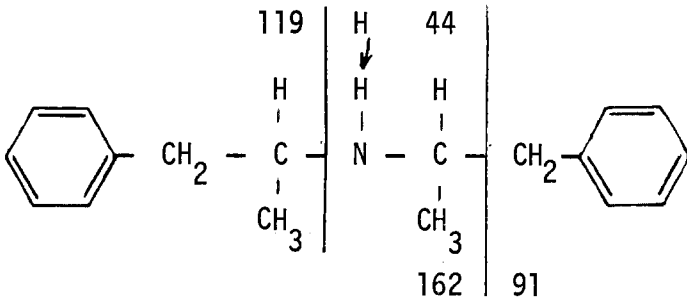
FIG. 5—The fragmentation scheme of di-(1-isopropylphenyl)-amine.
