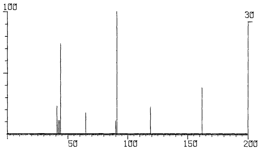
FIG. 4—The mass spectrum of di-(1-isopropylphenyl)-amine.
