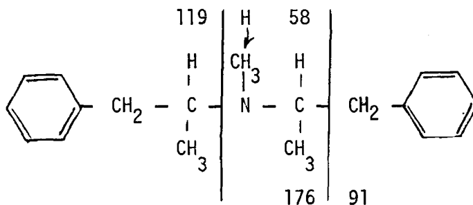
FIG. 13—The fragmentation scheme of di-(1-isopropylphenyl)-methylamine.
