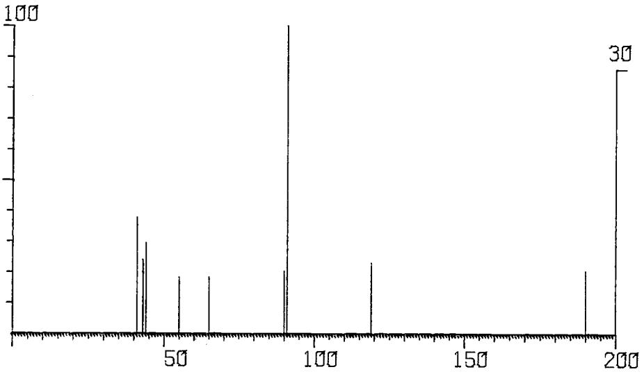
FIG. 6—The mass spectrum of tri-(1-isopropylphenyl)-amine.
