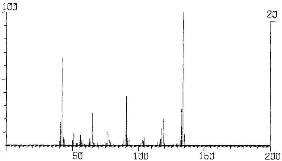
FIG. 11—The mass spectrum of a phenyl-2-propanone derivative.
